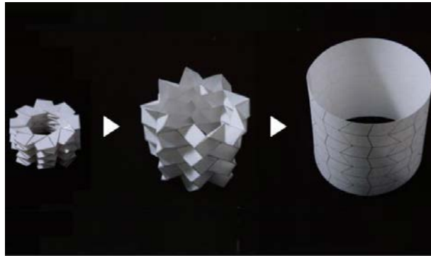
“SOGAME-ORI” Basic technology invented by SOGAME who is researcher for space architecture at Tokai univ.
